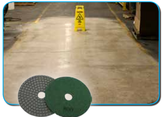
FIGURE 5-D: 800 GRIT GREEN SNAP! DISKS AND IMAGE OF FLOOR AFTER 800 GRIT DISKS.
