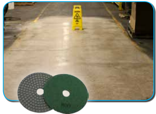
FIGURE 6-A: 800 GRIT GREEN SNAP! DISKS AND IMAGE OF FLOOR AFTER 800 GRIT DISKS.
